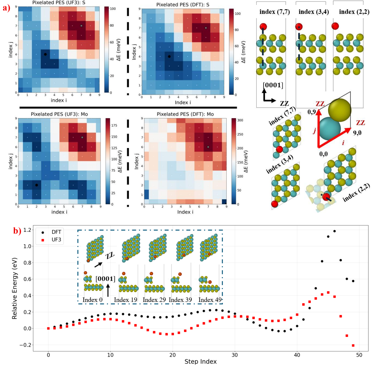
Fig. S5. (a) Sampled potential energy surface (PES) of S (top) and Mo (bottom) adatoms on the basal (0001) surface of 2H-MoS 2 predicted by UF3 (left) and DFT (right). The in-plane coordinates of the adatom were varied on a uniform 10 \times 10 grid spanning the lateral area of a single primitive surface unit cell (i.e., one surface translational period). The adatom height was fixed to a vertical displacement equal to the van der Waals gap in bulk 2H-MoS 2 , and the total energy of each configuration was normalized relative to the minimum energy sampled across the grid. The indices i and j denote the fractional in-plane coordinates of the adatom along the primitive lattice vectors, as illustrated schematically in the right panel. Each square of the pixelated grid is colored according to the value corresponding to the nearest sampled index pair. The minimum and maximum energy configurations are indicated by a black dot and gray star, respectively. Across the 100 sampled configurations, both UF3 and DFT predict that an S adatom positioned approximately above a Mo lattice site of the underlying layer (index (3,4)) corresponds to the lowest sampled energy, whereas positioning the adatom approximately above an S lattice site (index (7,7)) corresponds to the highest sampled energy. We note that indices (3,4) and (7,7) lie close to the lateral positions occupied by S and Mo atoms, respectively, in the next layer of ideal 2H-MoS 2 stacking, as illustrated in the right panel. The maximum normalized energy sampled for S adatoms is approximately 102 meV in UF3 and 106
